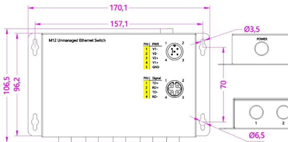
USR-ISF005-M12-CZ
