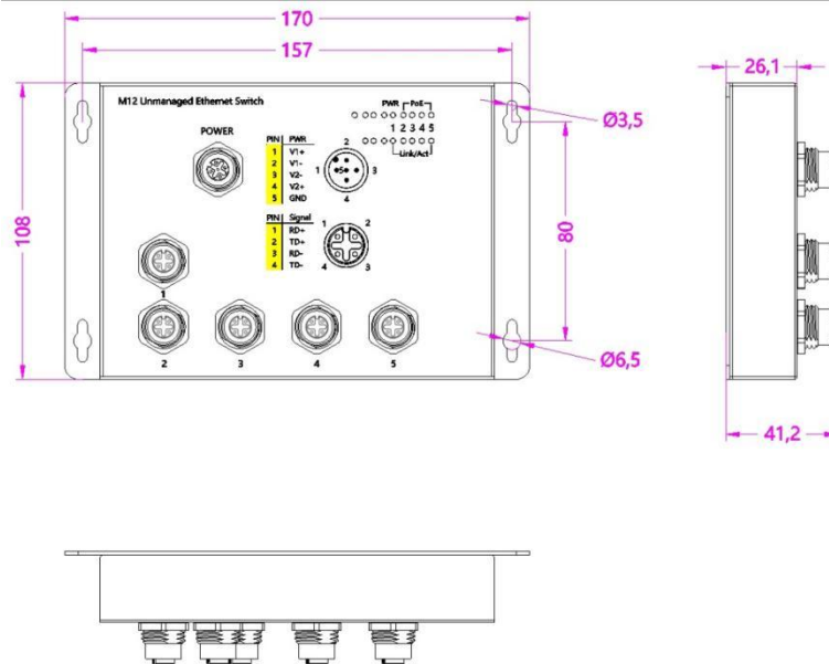
USR-ISF005-M12-BG
